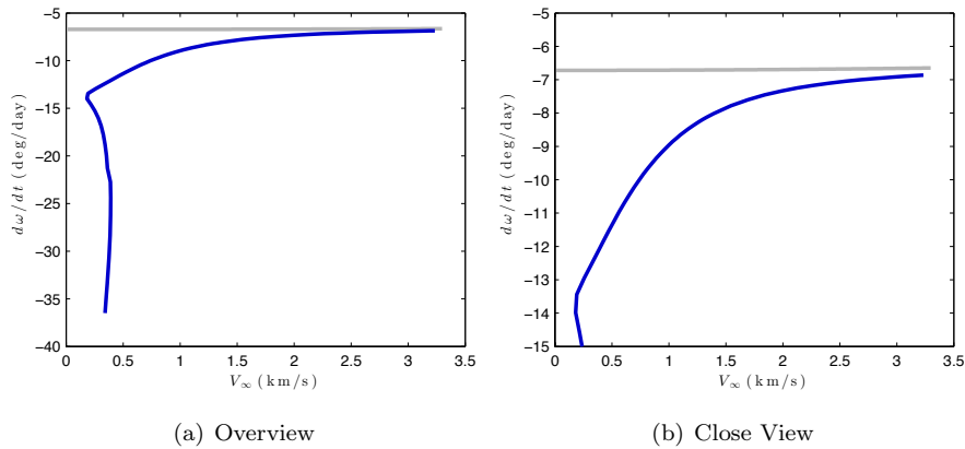
Figure 15. Comparison of the patched-conic \dot{\omega} (gray) and the CRTBP \dot{\omega} (blue) over a range of V_\infty values for the Jupiter-Europa 1:1 + /2:2 - sequence.
