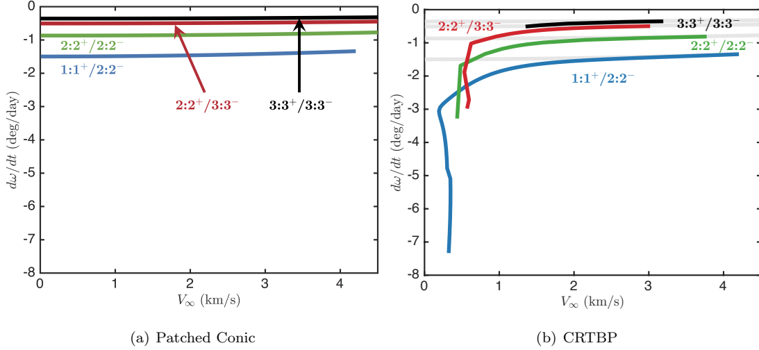
Figure 22. Patched-conic predictions and CRTBP results for \dot{\omega} in the Saturn-Titan system.
