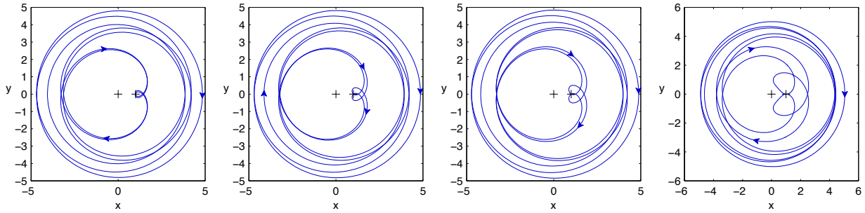
(a) V_\infty \approx 3.9 km/s, C \approx 2.92 (b) V_\infty \approx 5.0 km/s, C \approx 2.87 (c) V_\infty \approx 5.8 km/s, C \approx 2.83 (d) V_\infty \approx 10.3 km/s, C \approx 2.45
