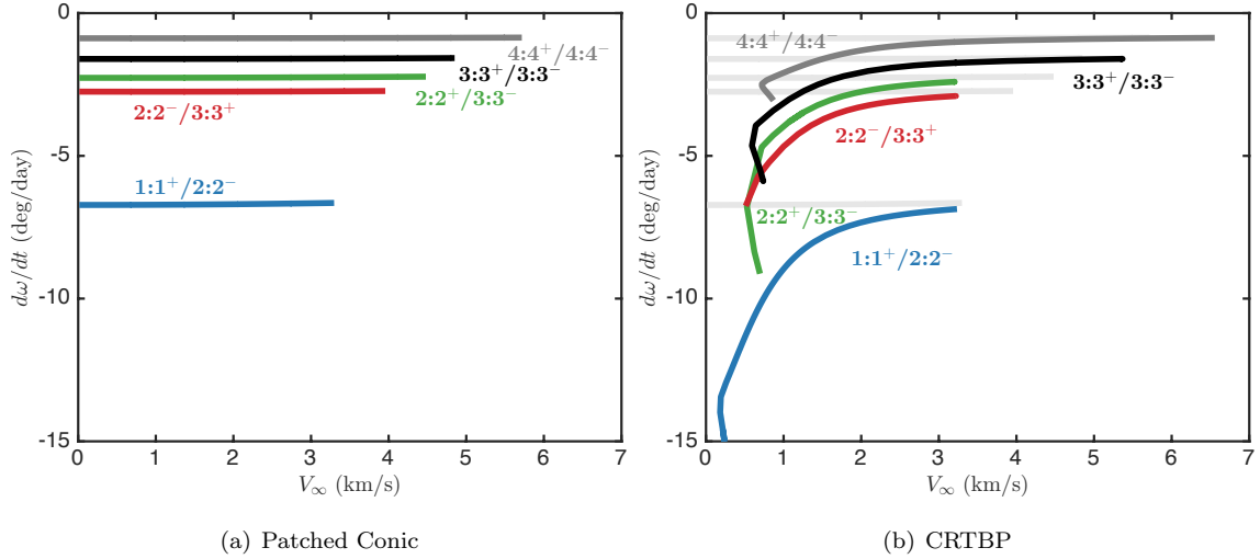
Figure 19. Patched-conic predictions and CRTBP results for \dot{\omega} in the Jupiter-Europa system for selected n:m^\pm/m:m^\mp orbits.
