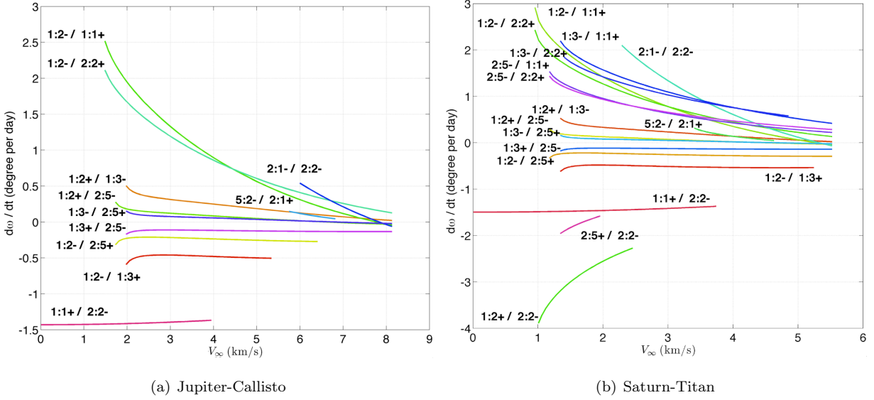
Figure 6. Rate of change of the argument of periaapse, \dot{\omega} , over V_\infty for the Jupiter-Callisto and Saturn-Titan dimensional cases.
