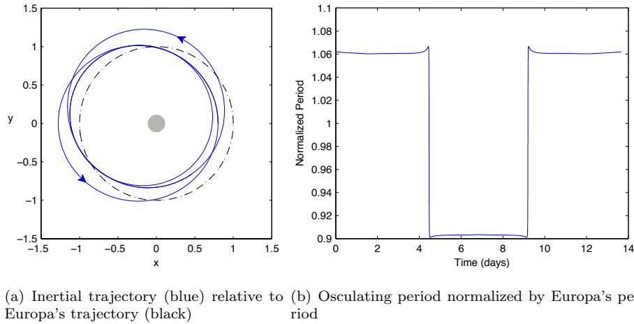
Figure 10. The converged three-body case in Figure 9(b) in the inertial frame and its period over time.
