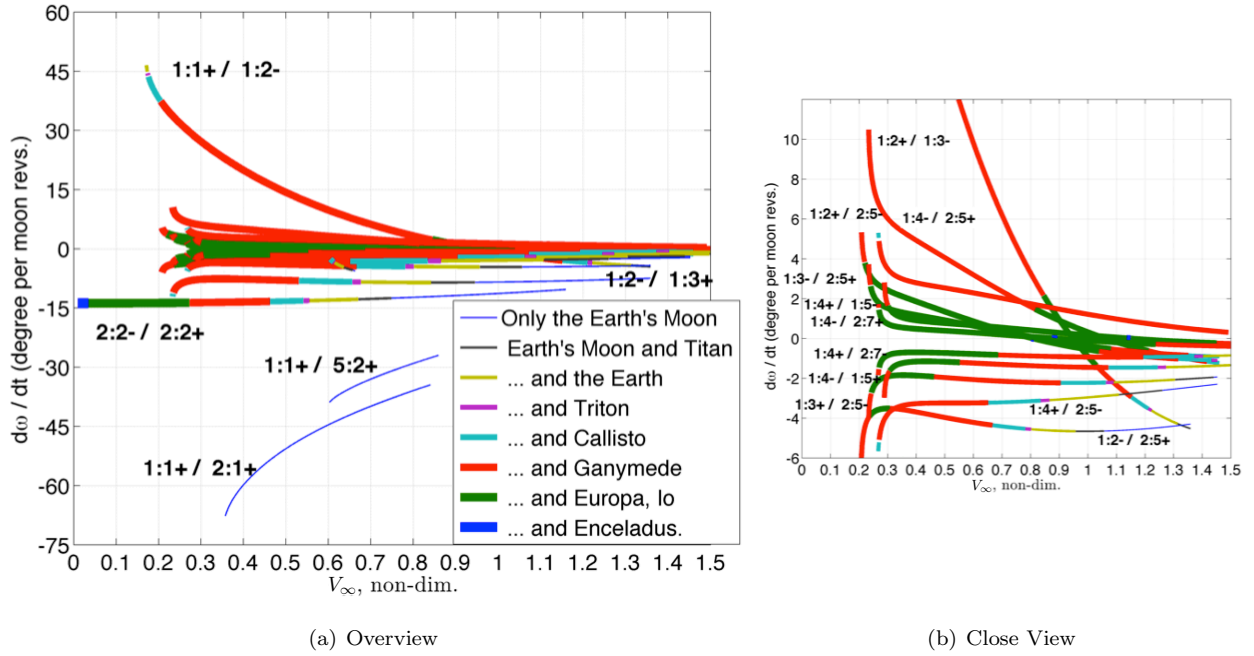
Figure 4. Rate of change of the argument of periapse, \dot{\omega} , across a range of dimensionless V_\infty values for a set of non-resonant orbit combinations.
