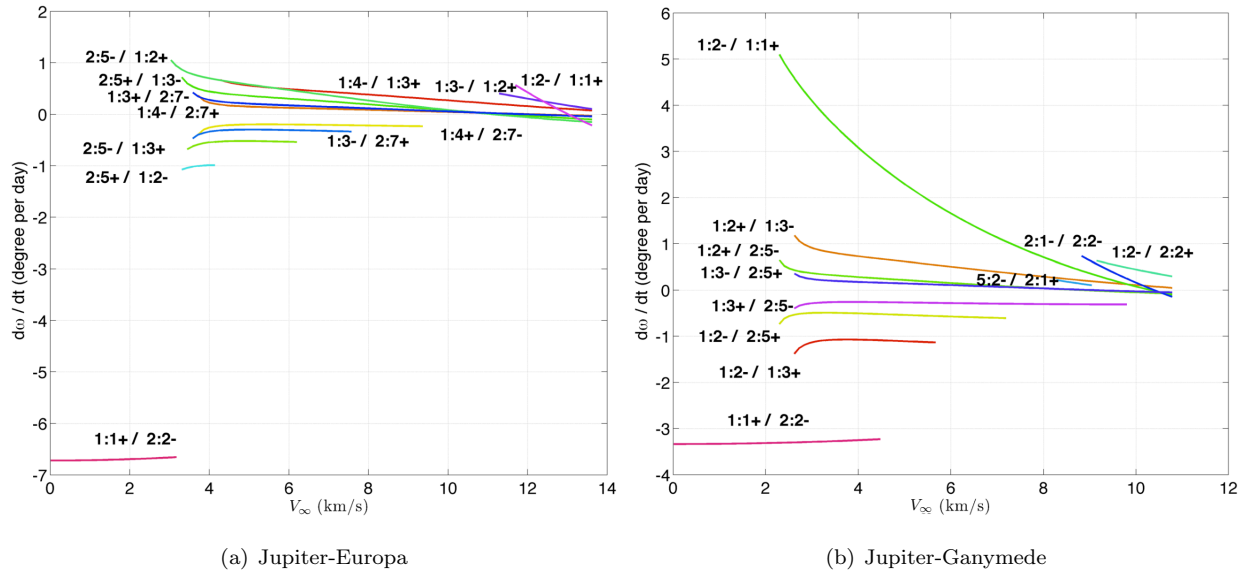
Figure 5. Rate of change of the argument of periapse, \dot{\omega} , over V_\infty for the Jupiter-Europa and Jupiter-Ganymede dimensional cases.
