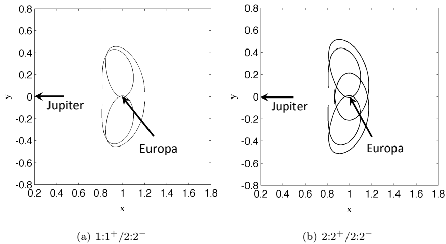
Figure 8. Two orbit cases with two-body initial conditions integrated in the CRTBP.
