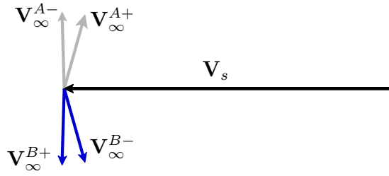
Figure 7. Diagram showing V_\infty vectors relative to the gravity assist body's velocity.
