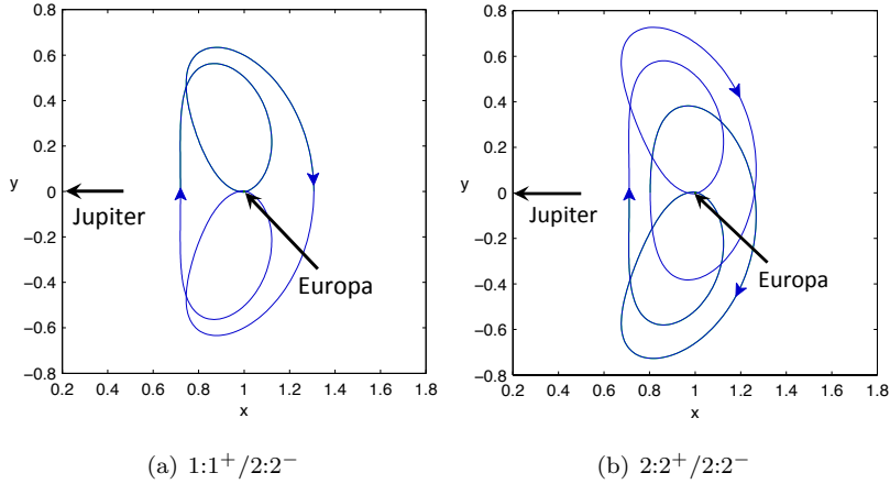
Figure 9. Converged three-body orbits plotted in the rotating Jupiter-Europa frame.
