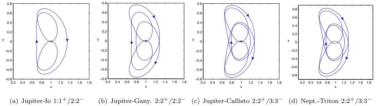
Figure 23. Sample of petal rotation trajectories for various non-resonant orbits and systems in the CRTBP.
