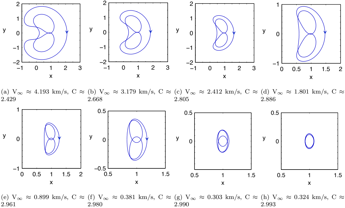
Figure 21. Sample of Saturn-Titan petal rotation trajectories across the continuation process for various 1:1^+/2:2^- orbits in the CRTBP.
