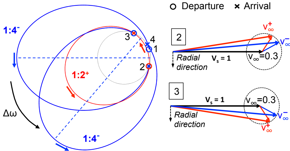
Figure 3. Petal strategy schematic for a 1:4^-/1:2^+ sequence with the rotation of the line of apsides.
