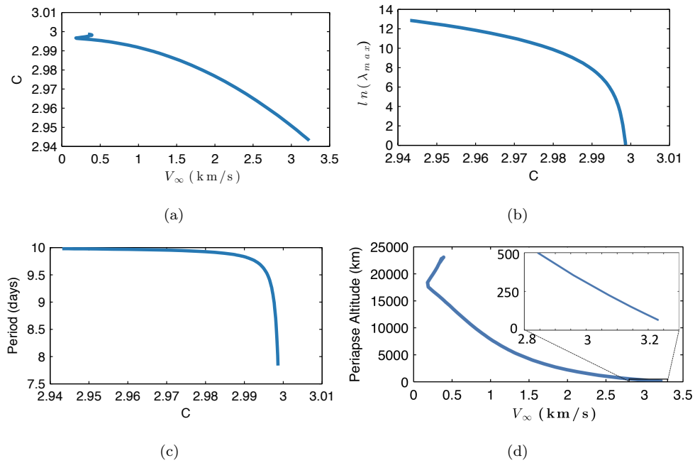
Figure 14. Characteristics of the Jupiter-Europa 1:1^+/2:2^- family across C and V_\infty .
