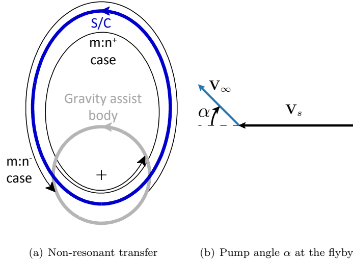
Figure 1. Illustration of possible non-resonant transfers including possible m:n^+ and m:n^- cases and the pump angle.
