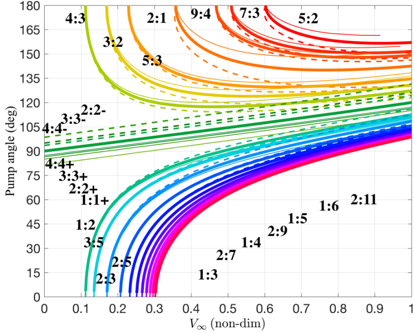
Figure 2. Pump angle across V_\infty for selected resonant and non-resonant orbits. The resonant (thick line), short non-resonant (dashed line), and long non-resonant (thin line) cases are shown.
