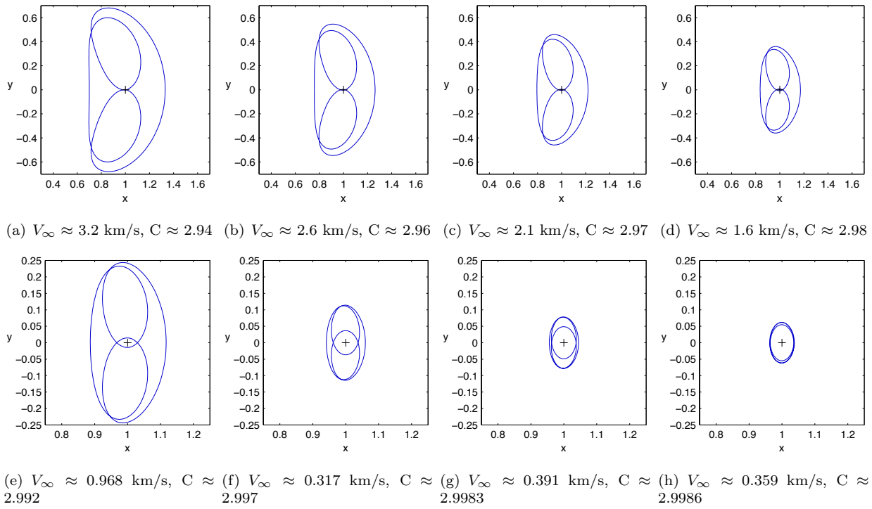
Figure 13. Selected trajectories from the Jupiter-Europa 1:1^+/2:2^- family.
