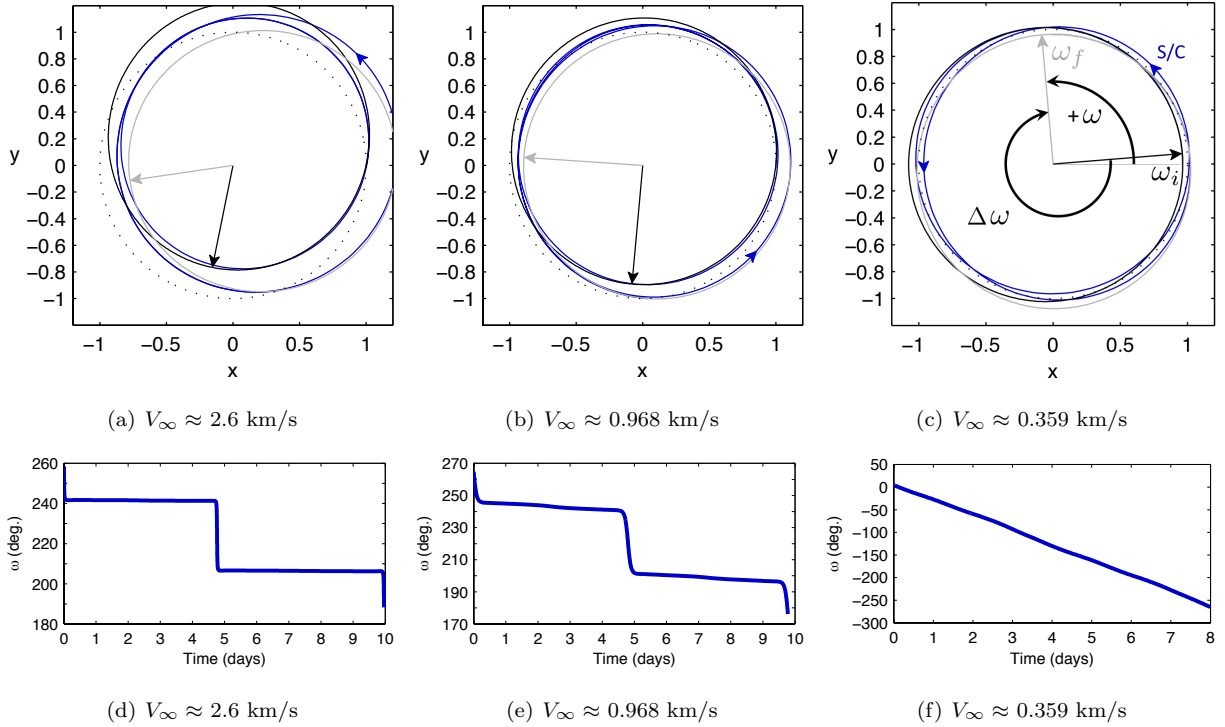
Figure 17. Selected trajectories from the 1:1^+/2:2^- sequence Figure 13 plotted in the inertial frame.
